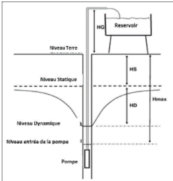
Charges hydrauliques
